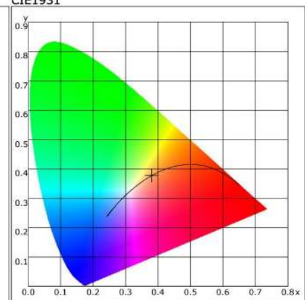
CIE1931
