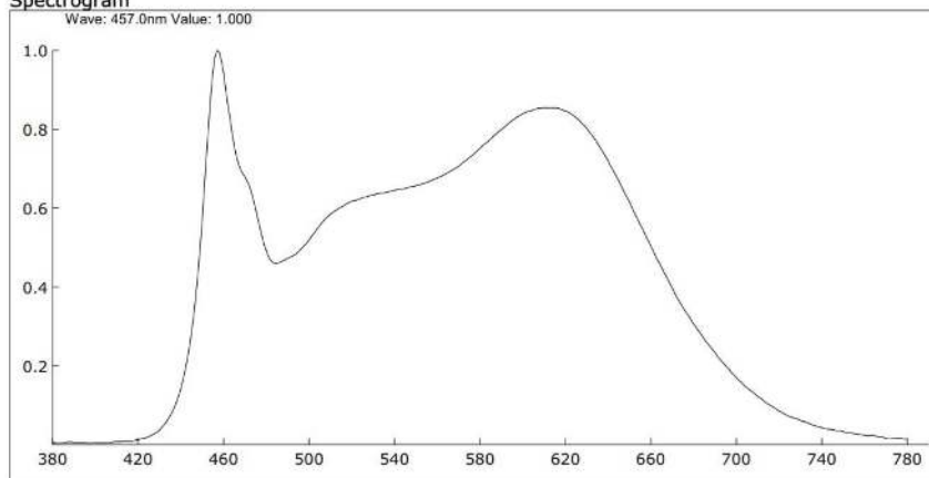
Spectrogram
