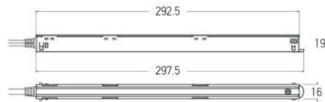
MAGNETIC TRACK 2085
