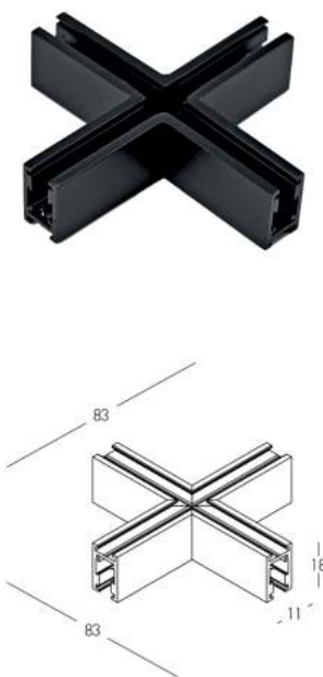
CROSS CONNECTOR (2515)
