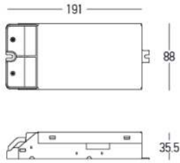
REMOTE DRIVER 150W ON-OFF / Code 20297
