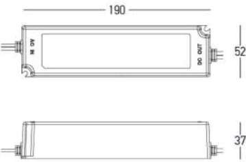
REMOTE DRIVER 100W ON-OFF / Code 20296
