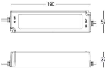
REMOTE DRIVER 100W ON-OFF / Code 20296
