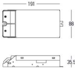
REMOTE DRIVER 150W ON-OFF / Code 20297
