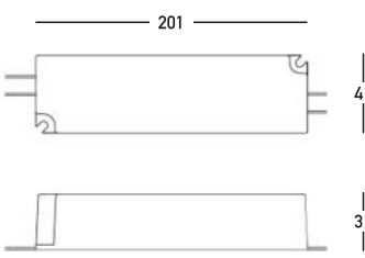
REMOTE DRIVER 100W ON-OFF / Code 25479
