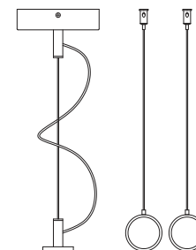
Suspension Kit 25105 (support 20-32W)
