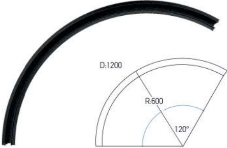
CURVED TRACK 120° D:1200MM (22103)
