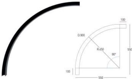
CURVED TRACK 90° D:900MM (22277)
