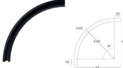
CURVED TRACK 90° D:600MM (22276)
