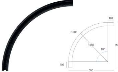
CURVED TRACK 90° D:900MM (22278)
