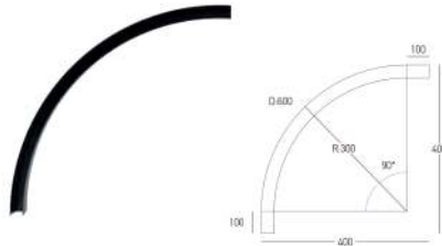
CURVED TRACK 90° D:600MM (22275)
