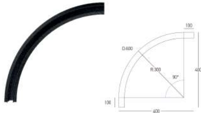
CURVED TRACK 90° D:600MM (22276)
