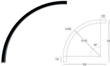
CURVED TRACK 90° D:900MM (22277)
