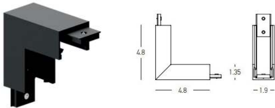
CORNER 90° VERTICAL (23132)
