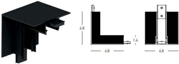
CORNER 90° VERTICAL (23133)
