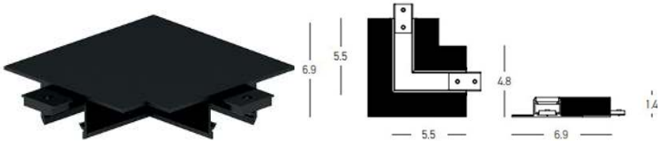
CORNER 90° HORIZONTAL (23130)
