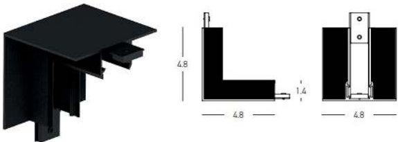
CORNER 90° VERTICAL (23133)
