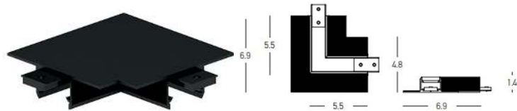
CORNER 90° HORIZONTAL (23130)
