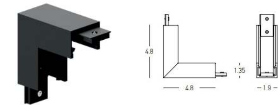
CORNER 90° VERTICAL (23132)
