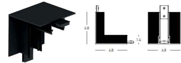
CORNER 90° VERTICAL (23133)
