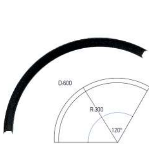
CURVED TRACK 120° D:600MM (22090)
