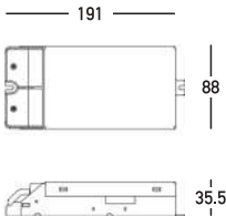
ON-OFF / Code 20297 DALI KIT / Code 20299 PUSH BUTTON KIT / Code 20302 BLUETOOTH KIT / Code 20305
