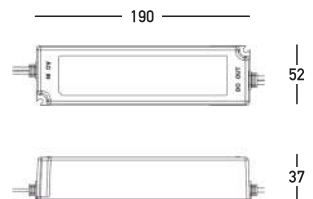
ON-OFF / Code 20296 DALI KIT / Code 20298 PUSH BUTTON KIT / Code 20301 BLUETOOTH KIT / Code 20304
