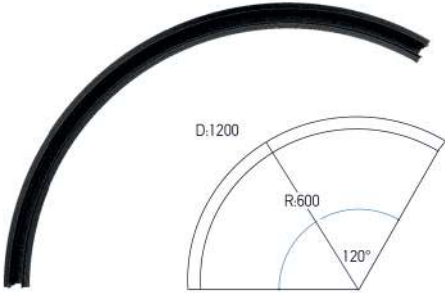
CURVED TRACK 120° D:1200MM (22103)
