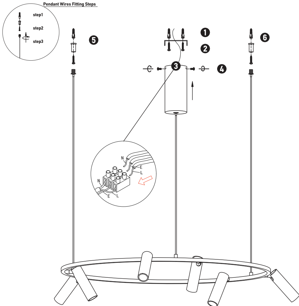
Pendant Wires Fitting Steps
