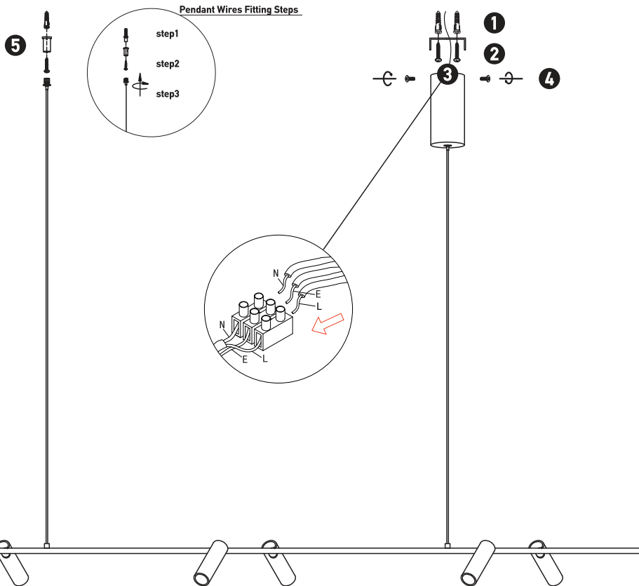
Pendant Wires Fitting Steps
